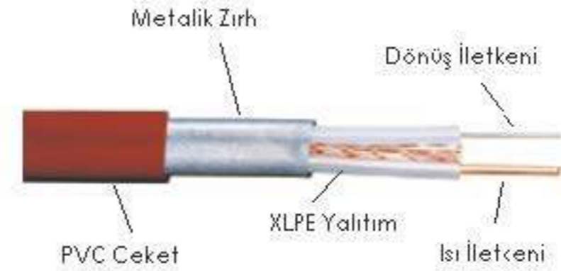
RAIL HEATER
