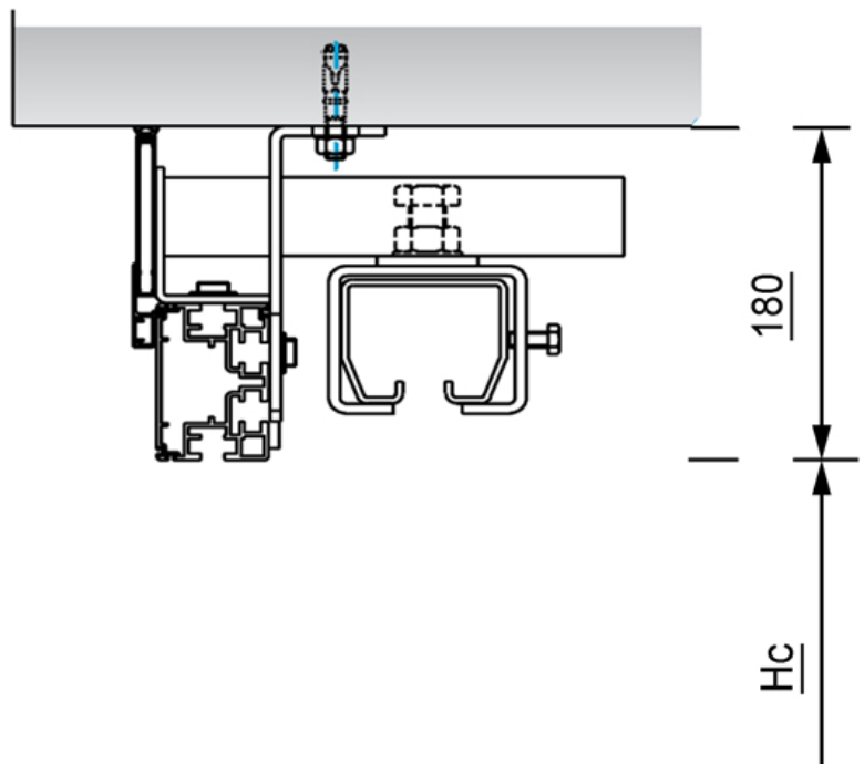
Installation into wall opening
